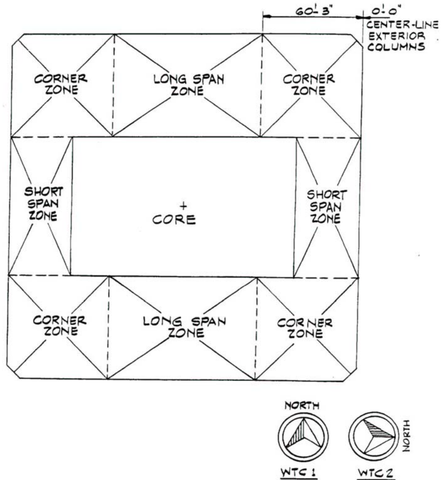
TYPICAL TENANT FLOOR PLAN ZONES FOR FLOOR NATURAL FREQUENCY MEASUREMENT FIGURE 2
