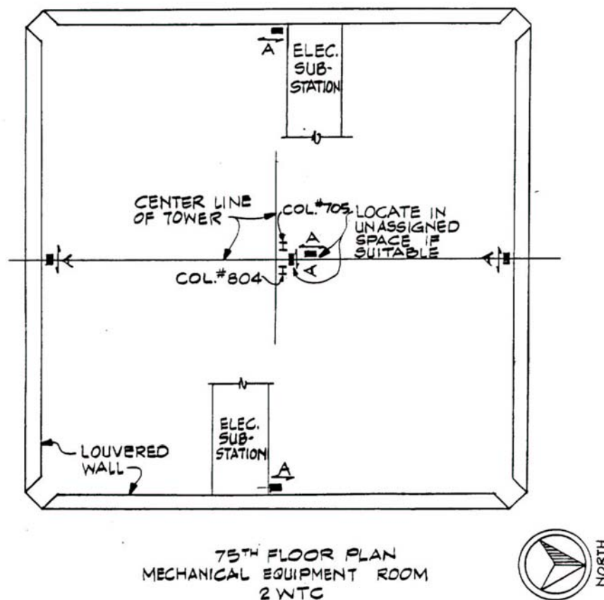
75 TH FLOOR PLAN MECHANICAL EQUIPMENT ROOM 2 WTC SUGGESTED LOCATIONS OF ACCELEROMETERS FOR MEASUREMENT OF TOWER NATURAL FREQUENCY
