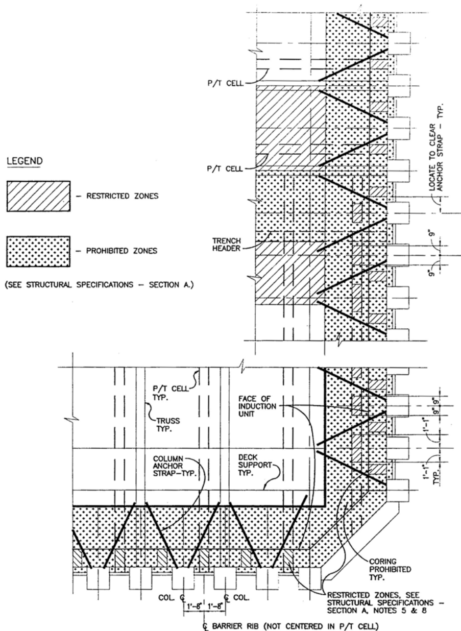
DETAIL AT BUILDING PERIMETER CORING CRITERIA
