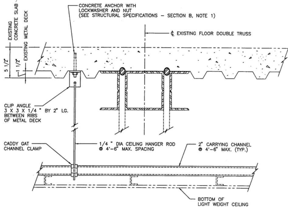
SECTION S-1
