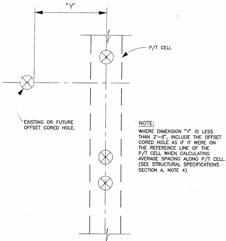
PLAN DETAIL OF SPACING CRITERIA AT OFFSET CORED HOLE CORING CRITERIA
