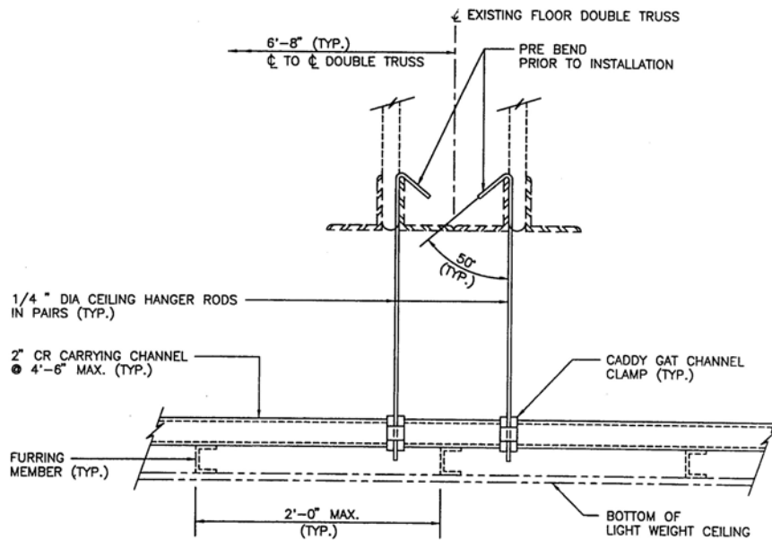
SECTION S-2 LIGHT WEIGHT CEILING SUPPORT SYSTEM FOR FLOORS W/DOUBLE TRUSSES
